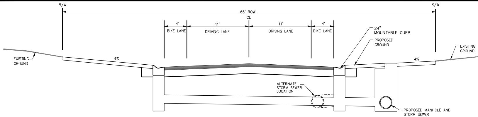
TOWN STANDARD TYPICAL URBAN SECTION WITH BIKE LANES STORM SEWER AT CATCH BASIN LOCATIONS – ALTERNATIVE OPTION U5 NO SCALE
