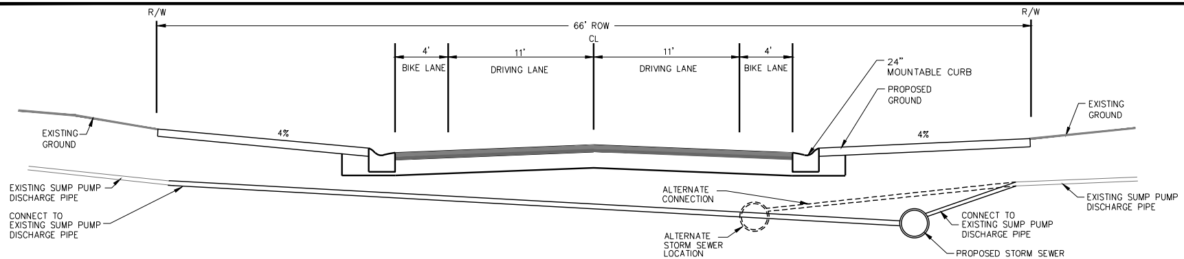
TOWN STANDARD TYPICAL URBAN SECTION WITH BIKE LANES STORM SEWER AT SUMP PUMP LOCATIONS – ALTERNATIVE OPTION U5 NO SCALE
