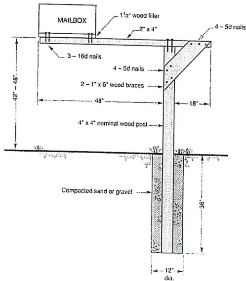
Figure 4: Example of a wood cantilever mailbox support
